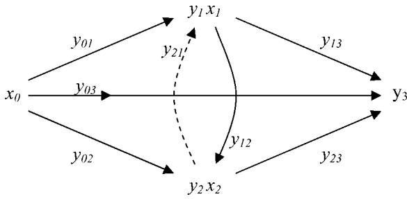
Figure 1 Two-relay network
